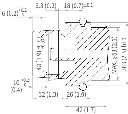
MAS 403 BT40
